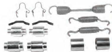
Brake Shoe Repair Kits (WAP) For Meritor 15" X 4" "Q" Plus Brake
