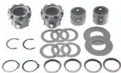
Camshaft Repair Kits (WAP) Eaton 12 1/4" Diameter, Late Model Brakes with M-2651 Spider
