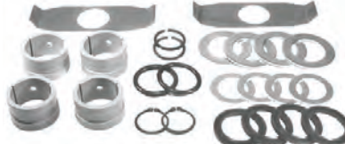
Camshaft Repair Kits (WAP) Meritor Axles Axles With 16 1/2" Diameter "Q" Brakes
